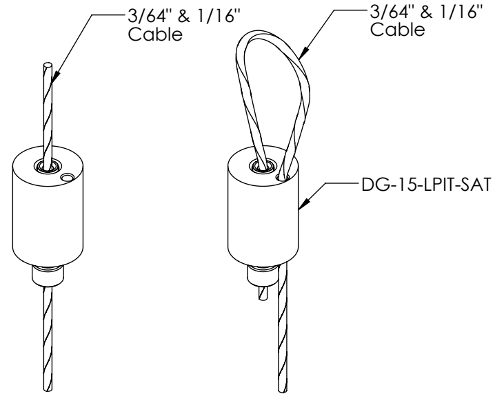
Adjustable Stop Configuration
